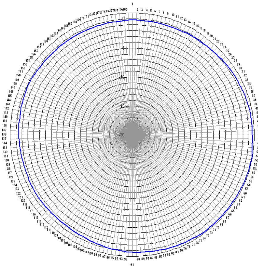
27.88GHz Omni Ant. H Pattern
